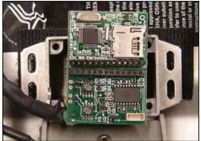
Photo courtesy of Marino di Marzo Components of the device, attached to the SCBA.
